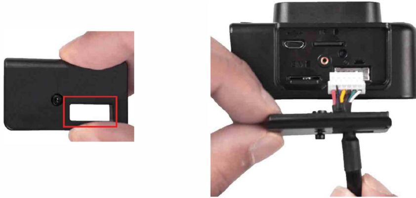
Feeding the 12-pin connector cable through the hole on the I/O cover
